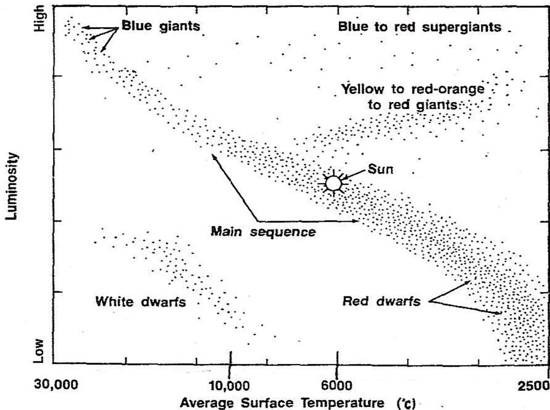
The Hertzsprung-Russell Diagram
